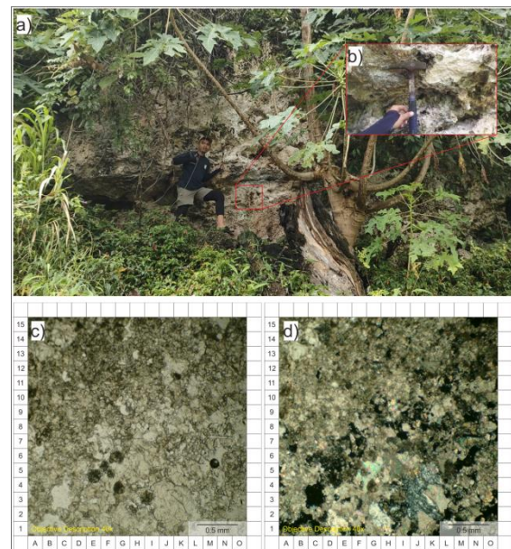
Gambar 5. a) Singkapan Batugamping Kristalin, b) Batugamping Kristalin, c) Sayatan Nikol Seajar, d) Sayatan Nikol Silang.
