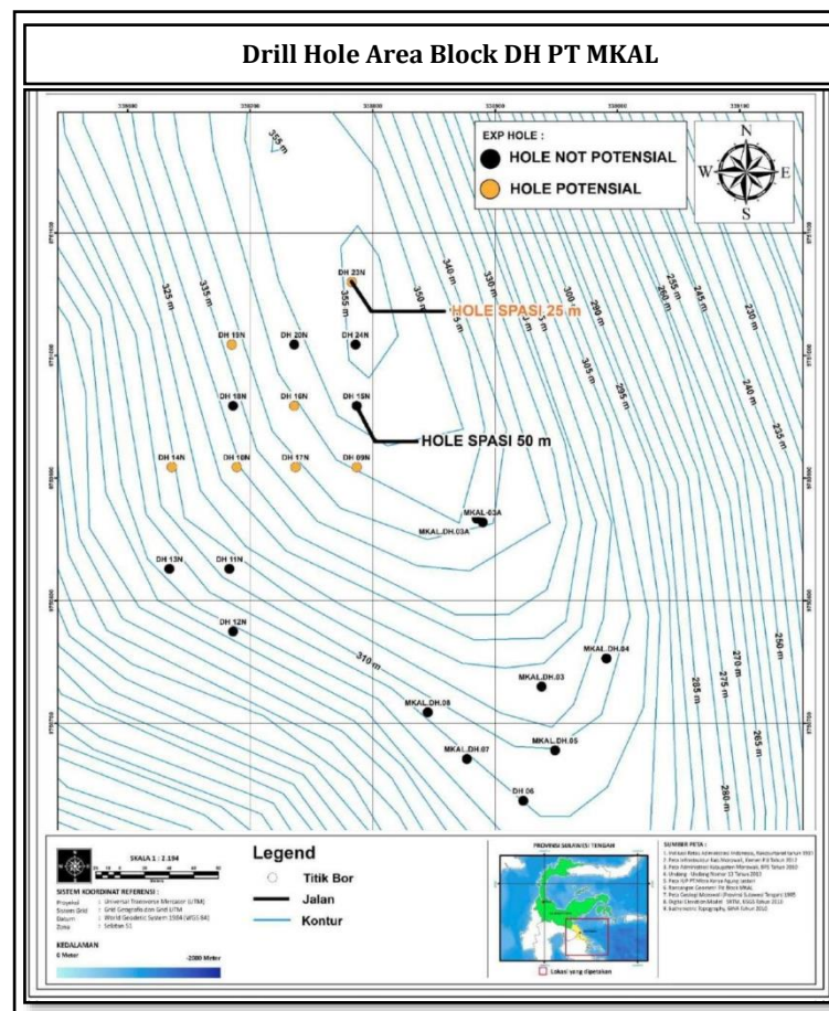
Figure 1. Drill Points Distribution.
