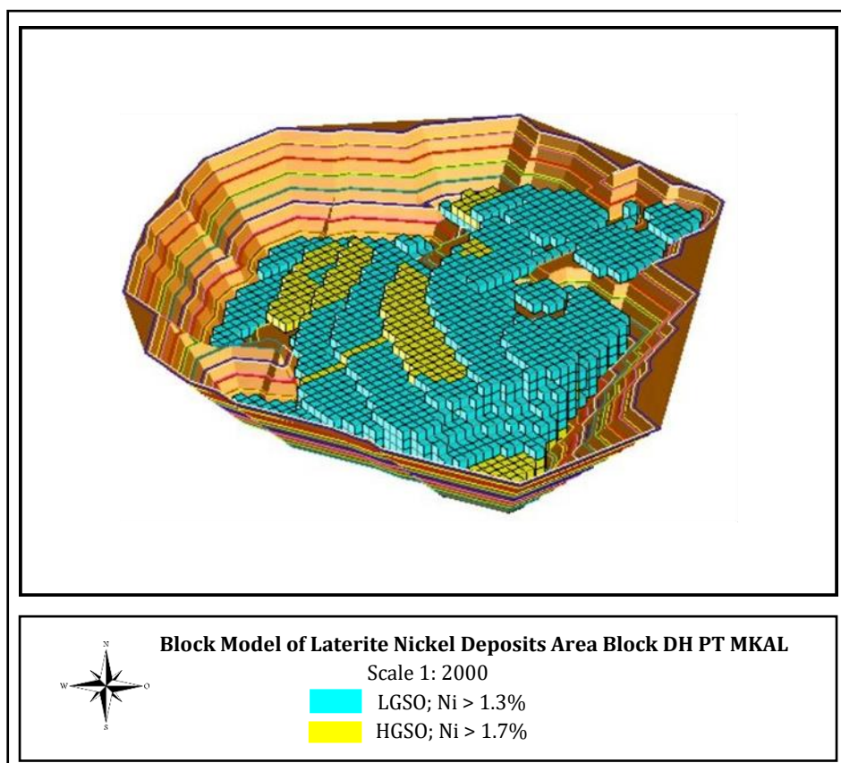
Figure 2. Block Model of Lateritic Nickel Deposits.
