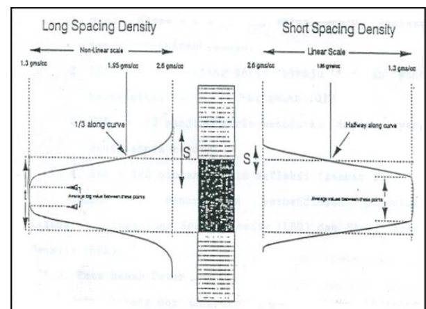
Gambar 4. Penentuan ketebalan antara log LSD (Long Spacing Density) dan SSD (Short Spacing Density) (BPB Manual, 1981).
