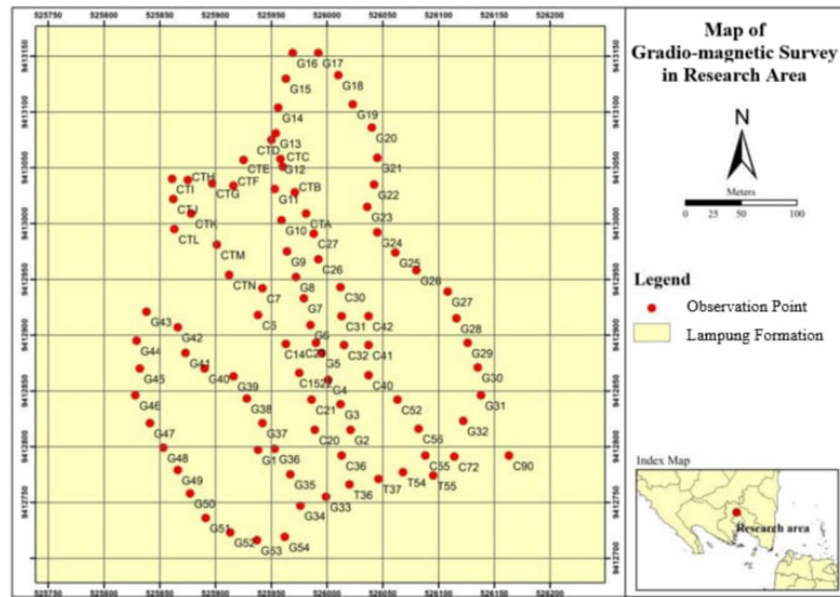
Figure 3. Design of the Cisarua Gradio-magnetic Survey.
