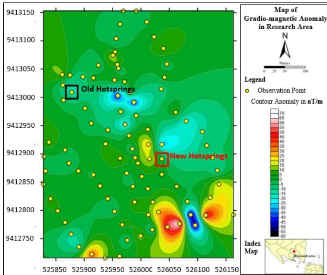
Figure 6. Gradio-magnetic Data Processing Result.
