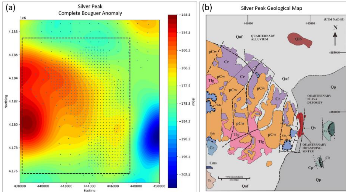
Figure 4. (a) Complete Bouguer Anomaly map of Silver Peak area. (b) Geological Map of Silver Peak area, modified from Hulen (2008) and Western Geothermal Partners LLC (2006). Note that the dashed-line rectangular on the CBA map denotes the covered area of the geological map.
