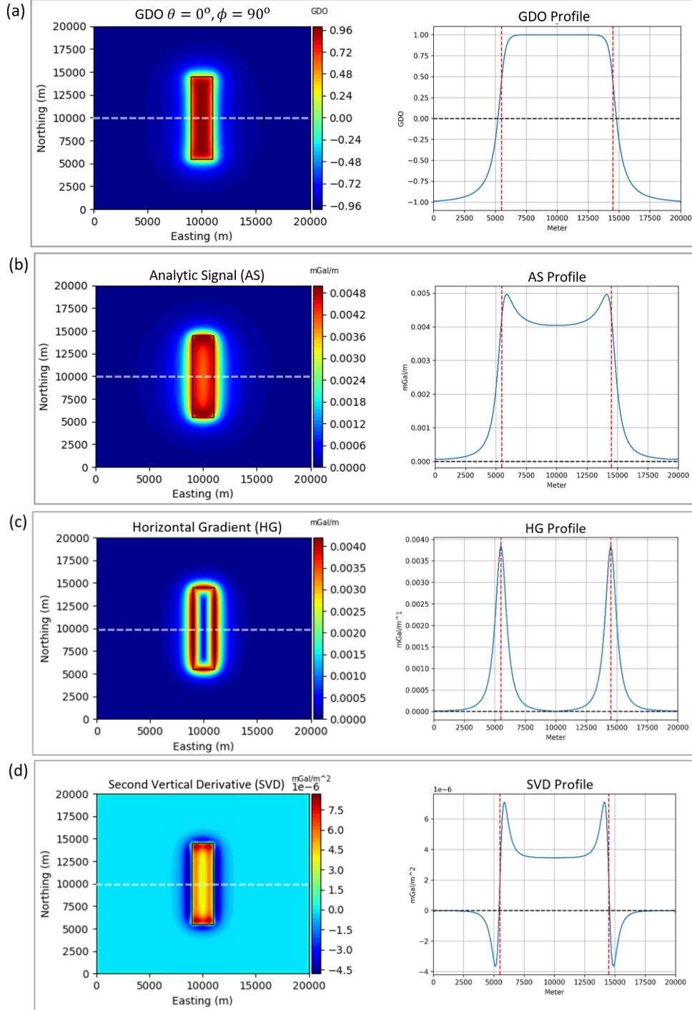
Figure 6. Results comparison of (a) GDO \theta = 0^\circ and \phi = 90^\circ , (b) Analytic Signal Amplitude (AS), (C) Horizontal Gradient (HG), (D) Second Vertical Derivative (SVD) based on local anomaly of synthetic model A. On the profile, red-dashed lines denote the edge of the prism and black-dashed line is zero value level.
