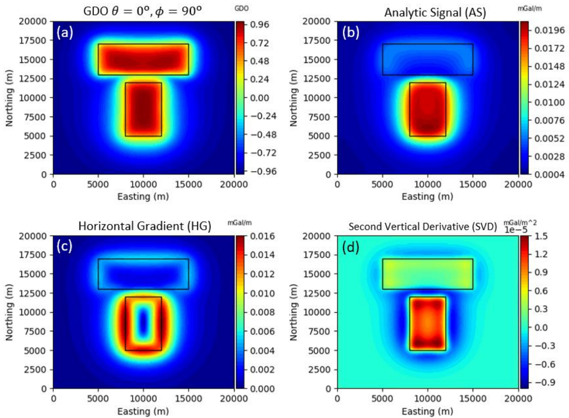
Figure 7. Results comparison of (a) GDO \theta = 0^\circ and \phi = 90^\circ , (b) Analytic Signal Amplitude (AS), (c) Horizontal Gradient (HG), (d) Second Vertical Derivative (SVD) based on regional anomaly of synthetic model B.
