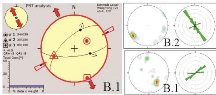
Figure 7. Stereograph analysis of the fracture data from station B.1 and B.2.
